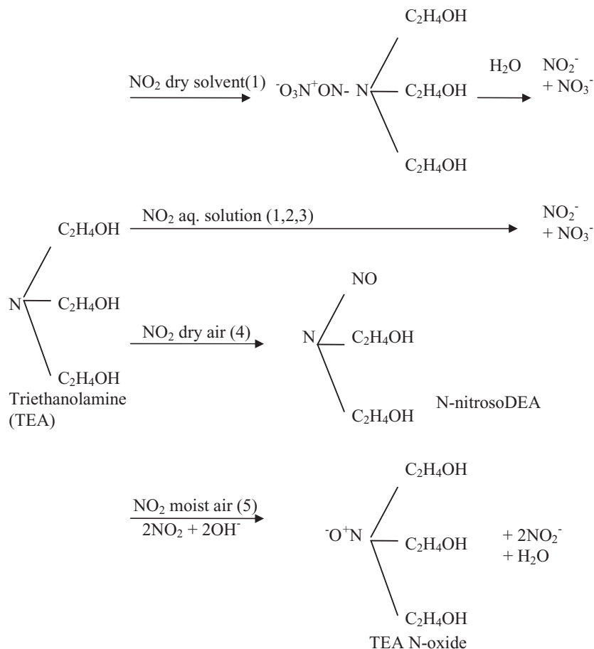
FIG. 3. Schematic of possible reactions of TEA with \text{NO}_2 with different products depending on conditions of reaction. Specific references are: 1) Gold (57); 2) Li et al. (63); 3) Wei et al. (65); 4) Aoyama and Yashiro (62); Brown (2); 5) Glasius et al. (64).
