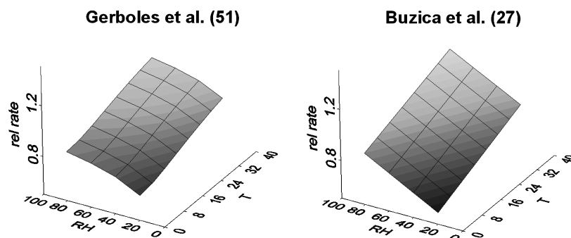
FIG. 2. Variation of sampling rate with temperature ( T , °C) and relative humidity (RH, %) based on dependence on [H_2O] [Gerboles et al., (51) — on left] or T and RH [Buzica et al. (27) — on right]. Data are expressed relative to calculated rates at 1 m/s, 20°C and 60% RH so that they can be compared visually.
