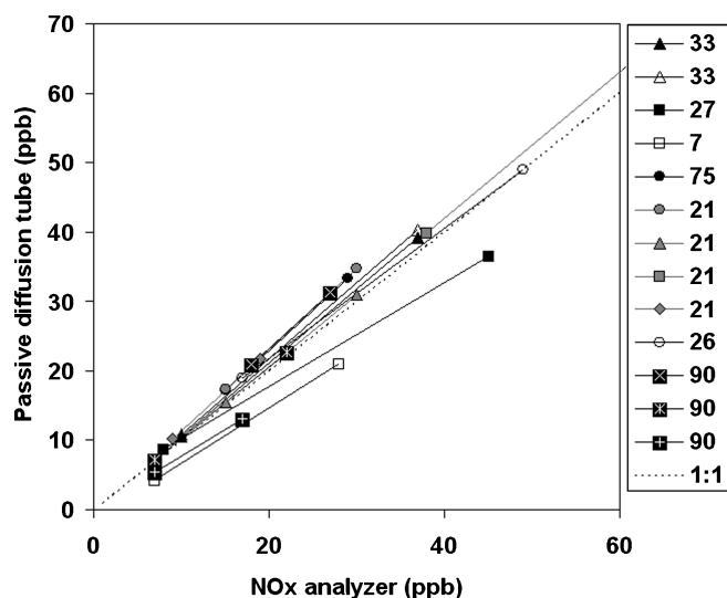
FIG. 5. Field comparisons of \text{NO}_2 concentrations measured using passive diffusion tubes exposed for 2 weeks with concentrations from a chemiluminescent \text{NO}_x analyzer (Table 5).
