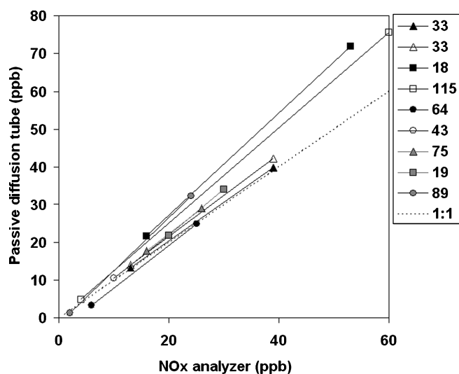
FIG. 6. Field comparisons of \text{NO}_2 concentrations measured using passive diffusion tubes exposed for 4 weeks with concentrations from a chemiluminescent \text{NO}_x analyzer (Table 6).
