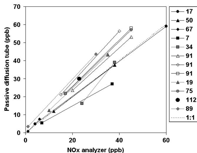
FIG. 4. Field comparisons of \text{NO}_2 concentrations measured using passive diffusion tubes exposed for 1 week with concentrations from a chemiluminescent \text{NO}_x analyzer (Table 4).
